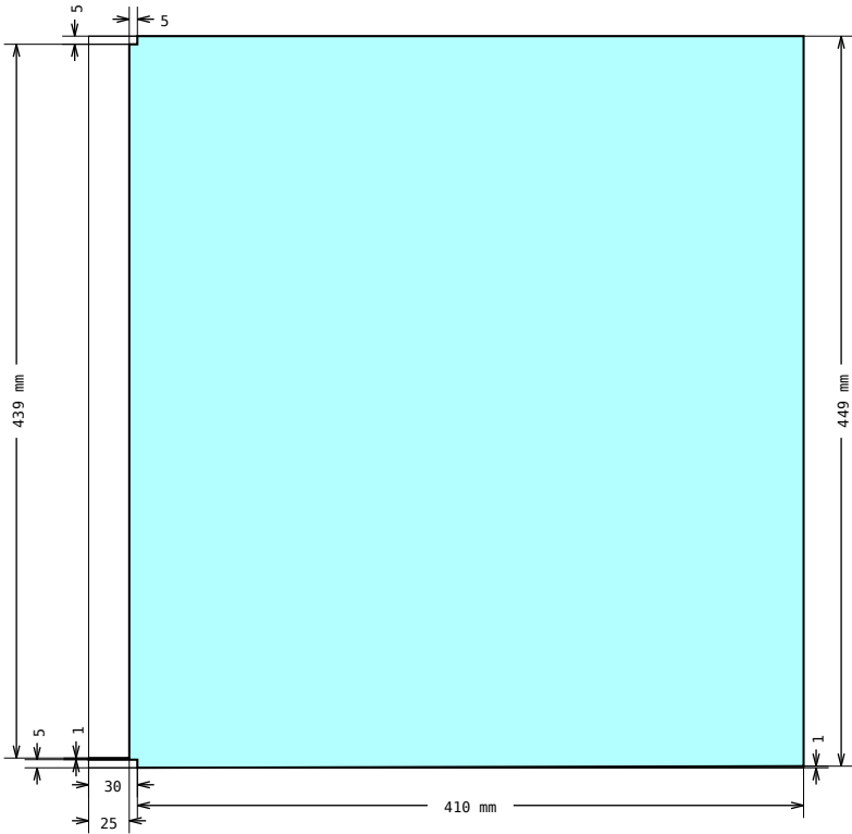
DRAWING 8, Pos 27 Shape measurements
