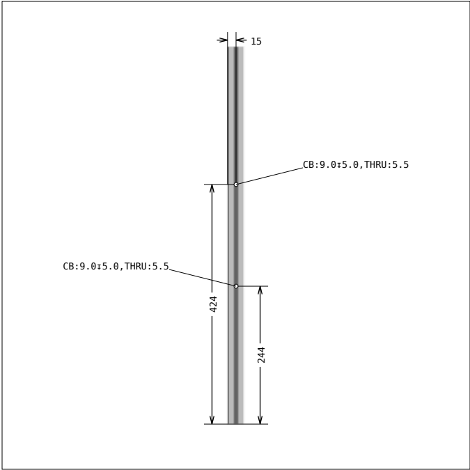
DRAWING 1, Pos 8 SIDE 4
