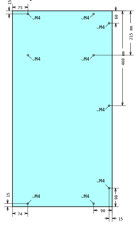
DRAWING 13, Pos 32 Hole placement
