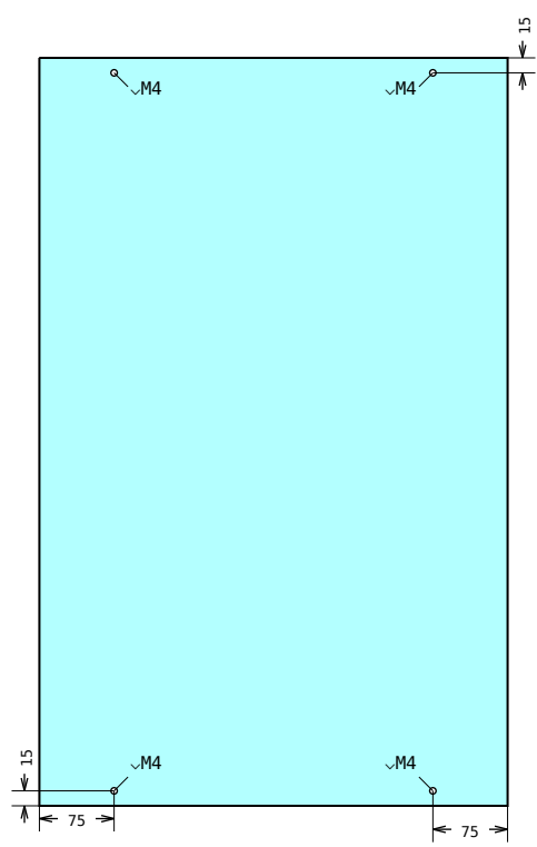
DRAWING 11, Pos 30 Hole placement
