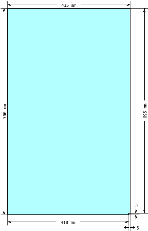
DRAWING 10, Pos 29 Shape measurements
