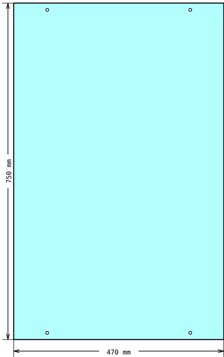
DRAWING 11, Pos 30 Shape measurements
