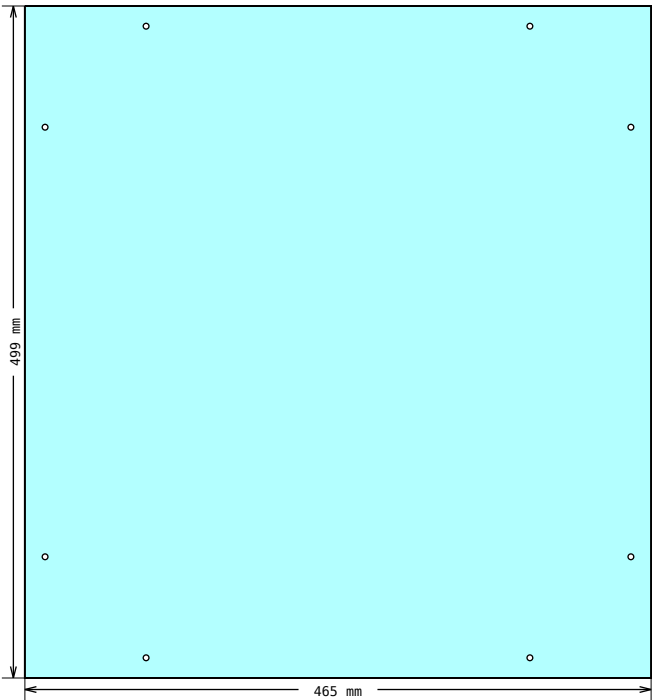
DRAWING 9, Pos 28 Shape measurements
