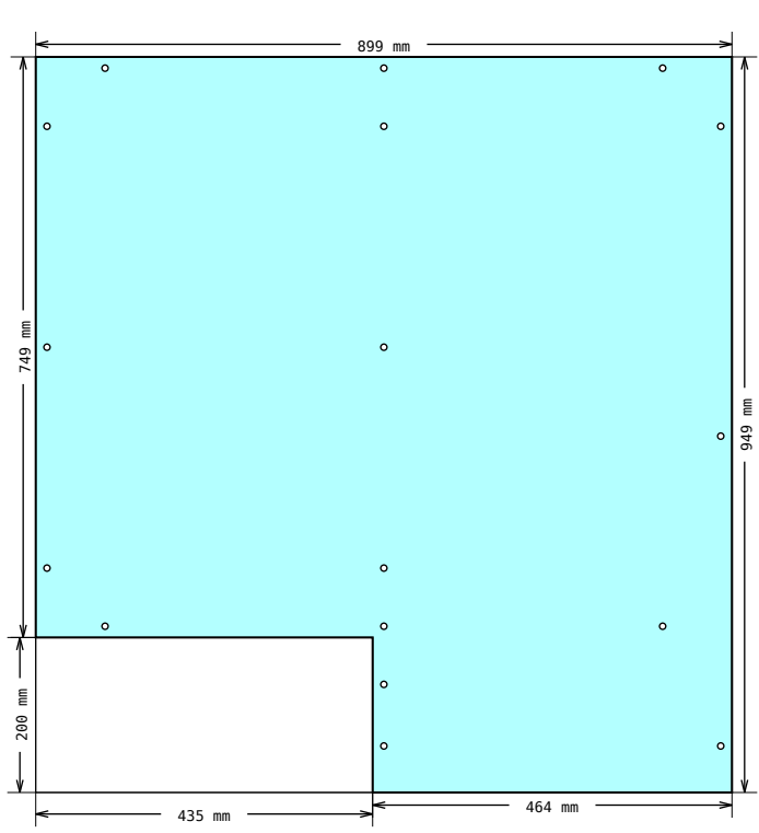
DRAWING 14, Pos 33 Shape measurements
