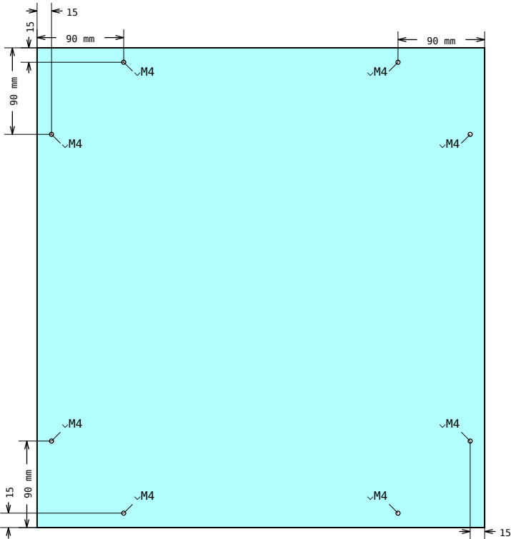
DRAWING 9, Pos 28 Hole placement
