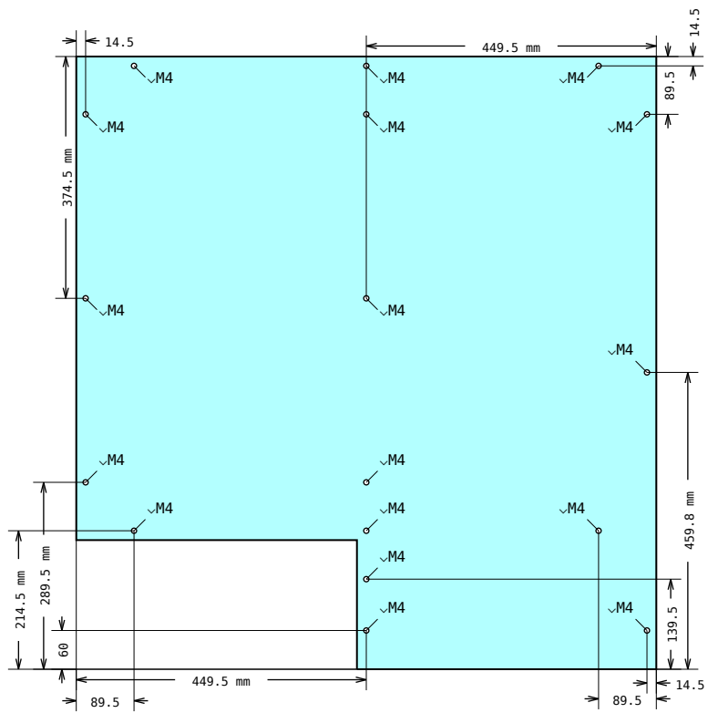
DRAWING 14, Pos 33 Hole placement
