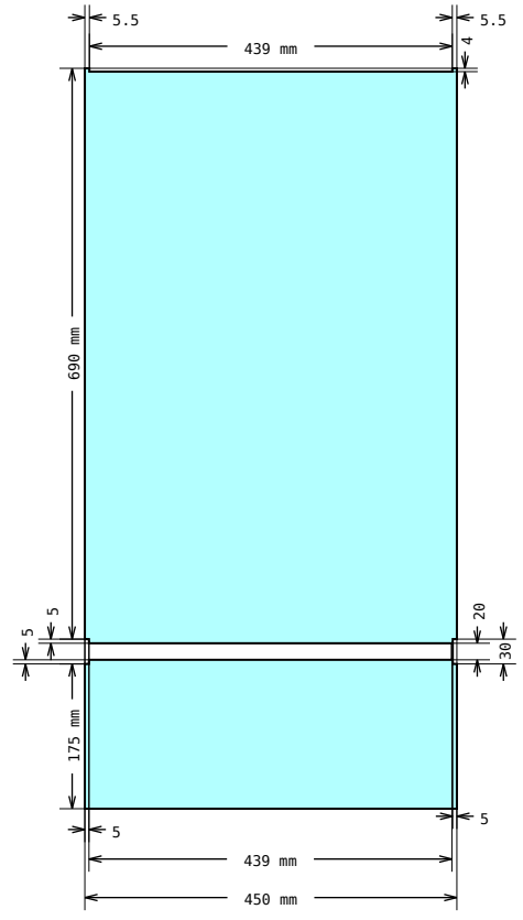
DRAWING 12, Pos 31 Shape measurements
