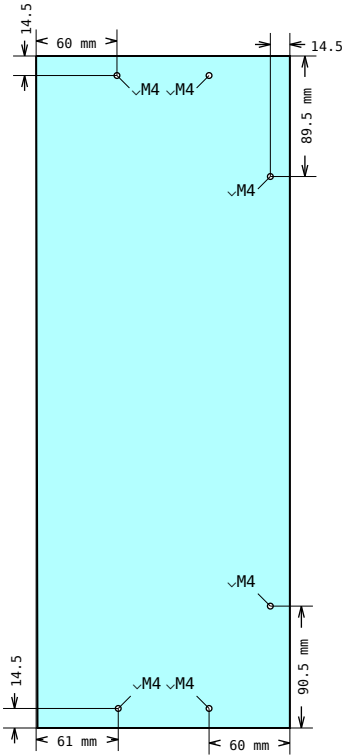
DRAWING 6, Pos 25 Hole placement
