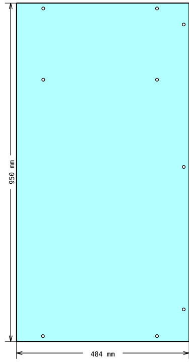
DRAWING 13, Pos 32 Shape measurements
